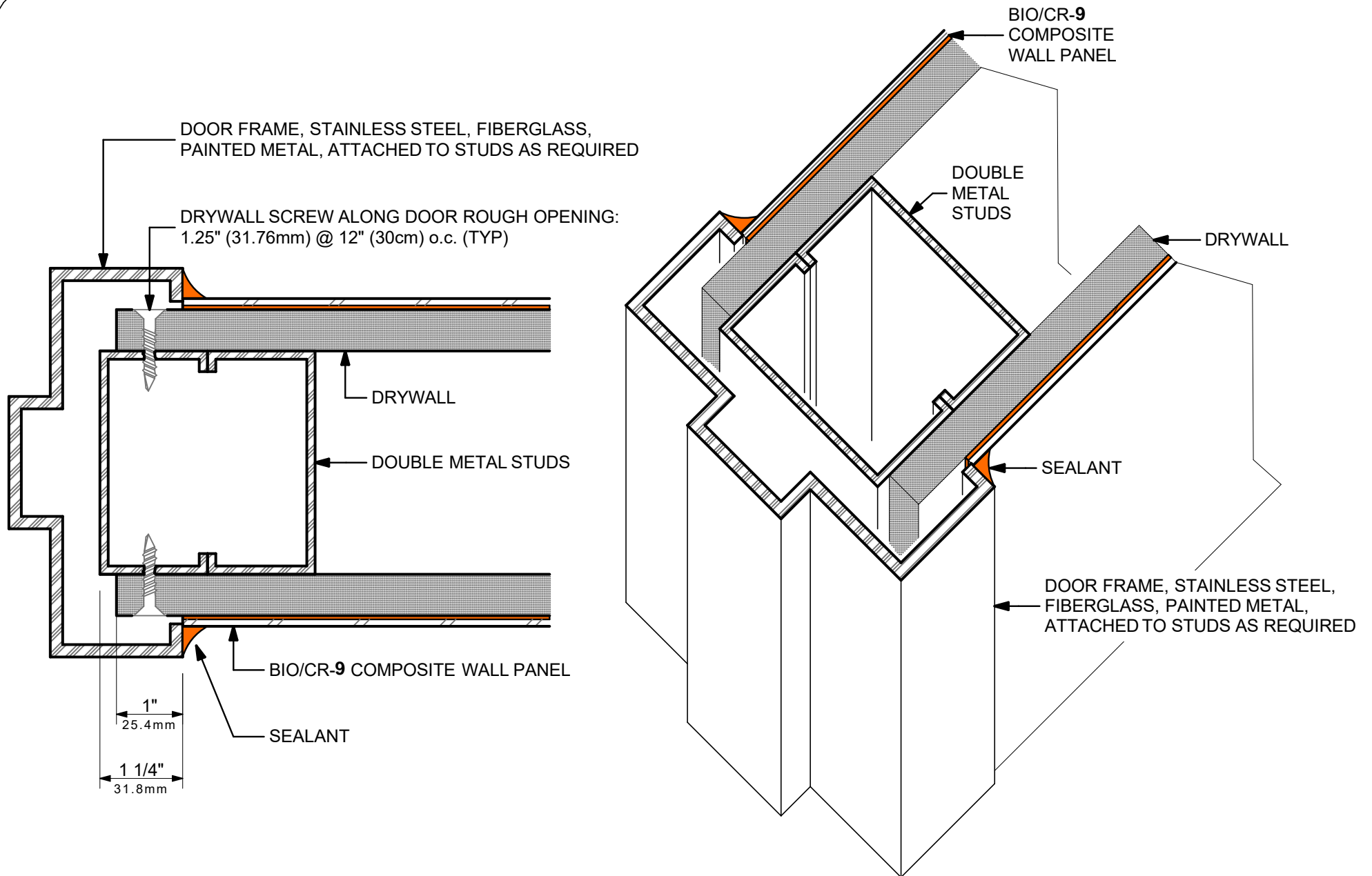
Bio/CR-9 DOOR FRAME SEALING DETAIL, TYPICAL JAMB (HEAD SIMILAR)
