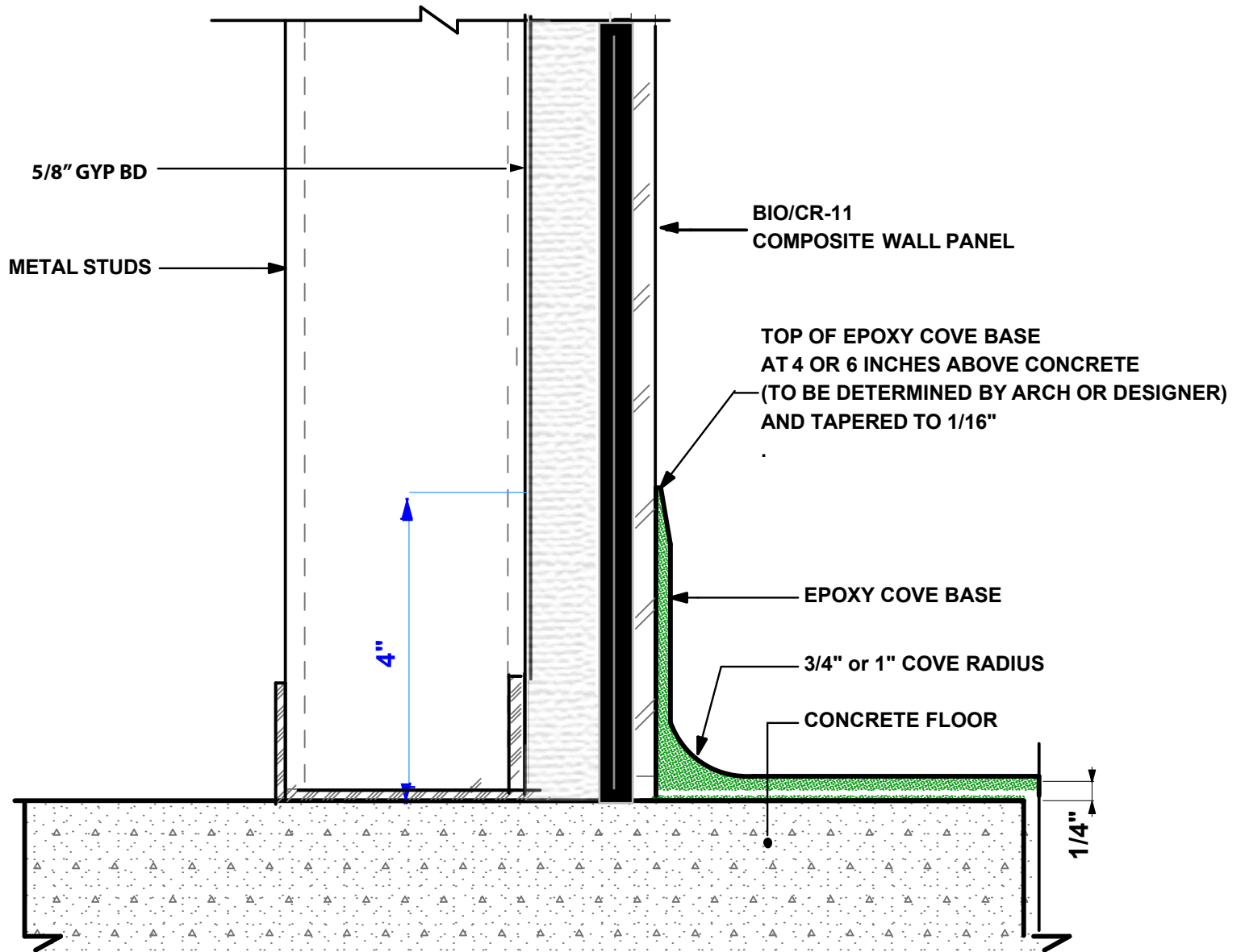
Bio/CR-11 (On Gyp) Clean Room Cove Base Detail w/ Tapered Cove Base
