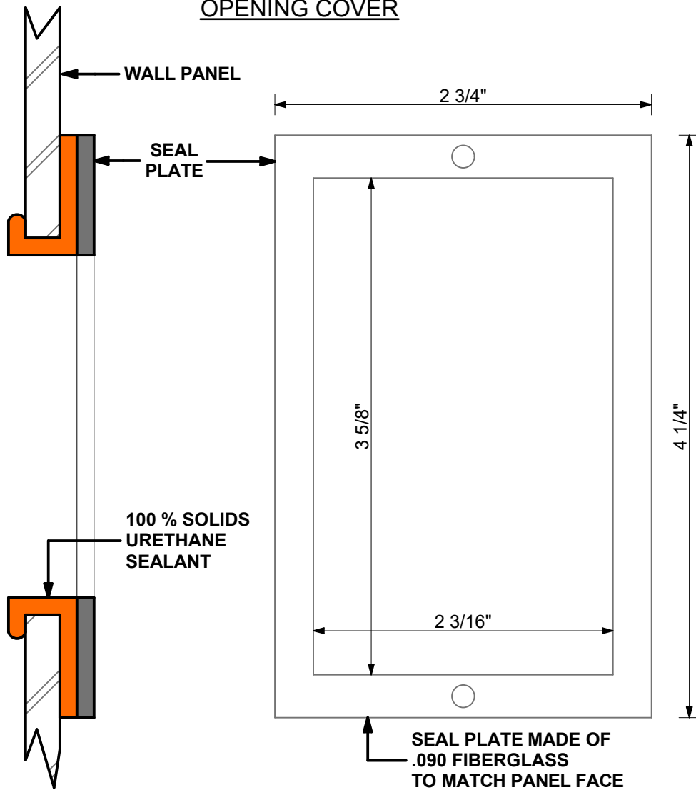
SIDE VIEW
