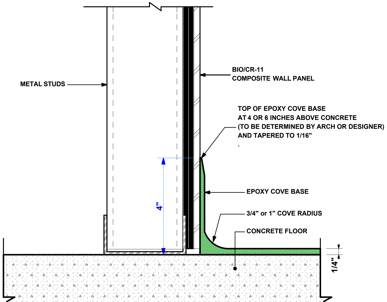
Bio/CR-11 Clean Room Cove Base Detail w/ Tapered Cove Base
