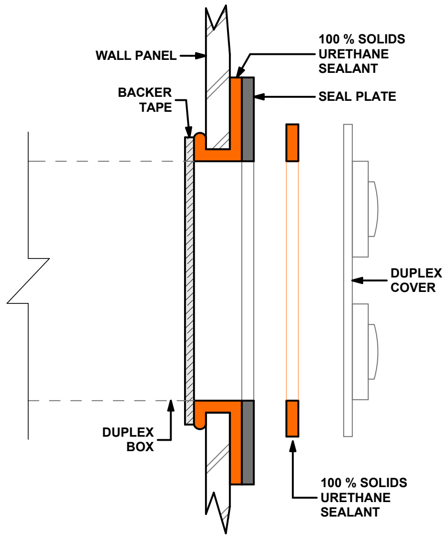
SIDE VIEW
